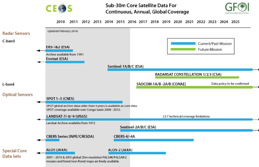
Figure 13: GFOI Initiative: sub-30 Core Satellite Data for Continuous, Annual, Global Coverage
