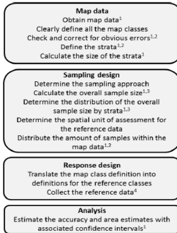
Figure 24: The main four steps of an accuracy assessment: Obtaining and finalising the map data, sampling design, response design and analysis. The symbols show the software that can accomplish that step: 1 is R, 2 is QGIS, 3 is Excel, and 4 is Collect Earth.
