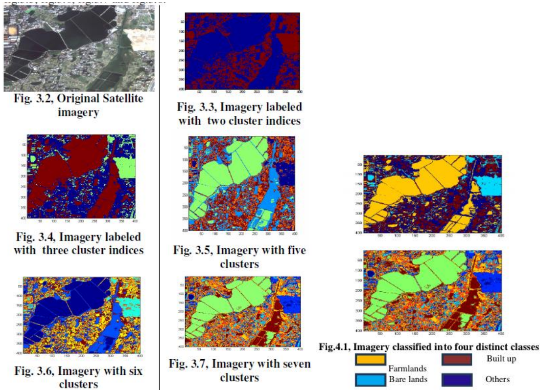
Figure 39: Example of k-means clustering of satellite data with different values of k. Clusters are classified into landuse types. Usman (2013).
