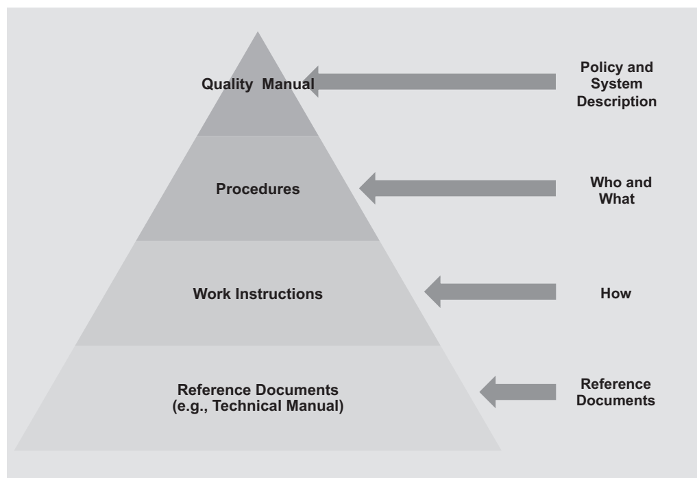
Figure 13.2 Documentation
